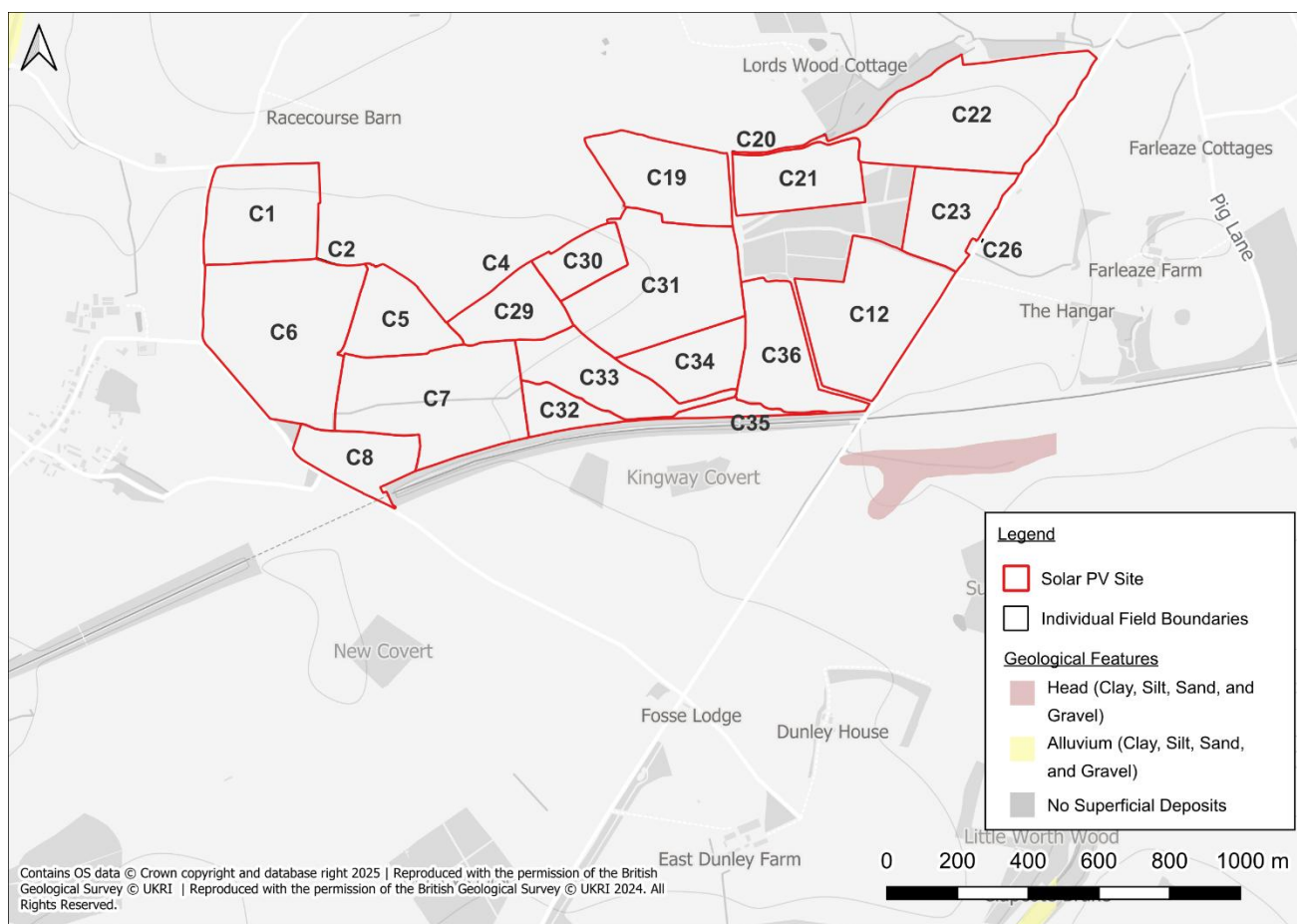
Figure 3: Superficial Deposits
